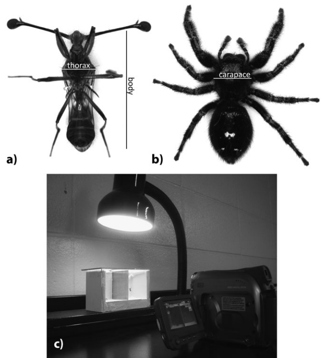
Figure 1 a) Male Teleopsis dalmanni lying on dorsal side for marked measurements of eye span, body length, and thorax width. (b) Arachnid predator Phidippus audax with marked measurement of carapace width. (c) Experimental set up of arena, lighting, and video camera.
